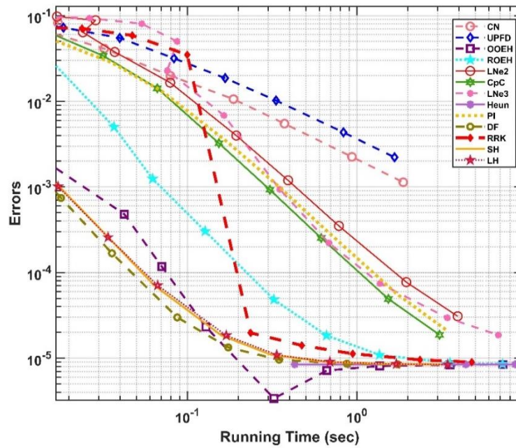
Figure 4.5. The maximum errors as a function of the running time for the 13 examined methods in the case of an equidistant mesh.
