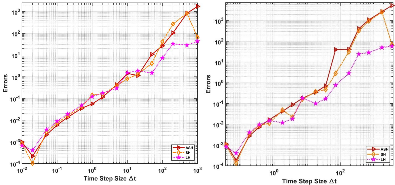
Figure 4.51. The maximum error as a function of time step size of three numerical methods for PCM1 (Left), and for PCM2 (Right).
