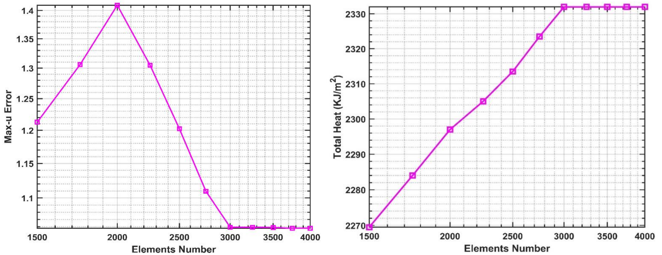
Figure 4.50. The mesh dependency examination, number of mesh elements with max error (Left), and with total penetrated heat (Right)
