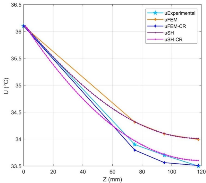
Figure 4.32. The temperature at the 4 selected measurement points in z at time t = 20 min.
