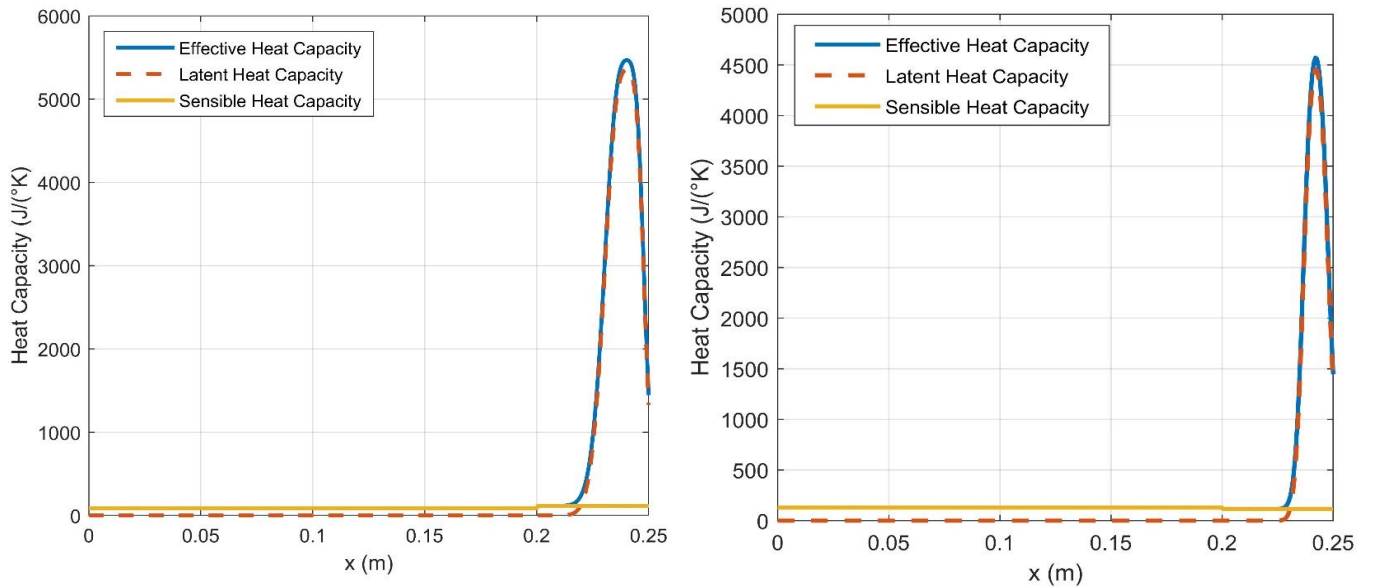
Figure 4.52. The heat capacity in Case1 for of Brick+PCM1 (Left), Concrete +PCM1 (Right)
