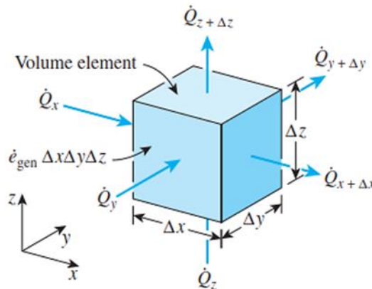
Figure 2.1. 3D rectangular element
