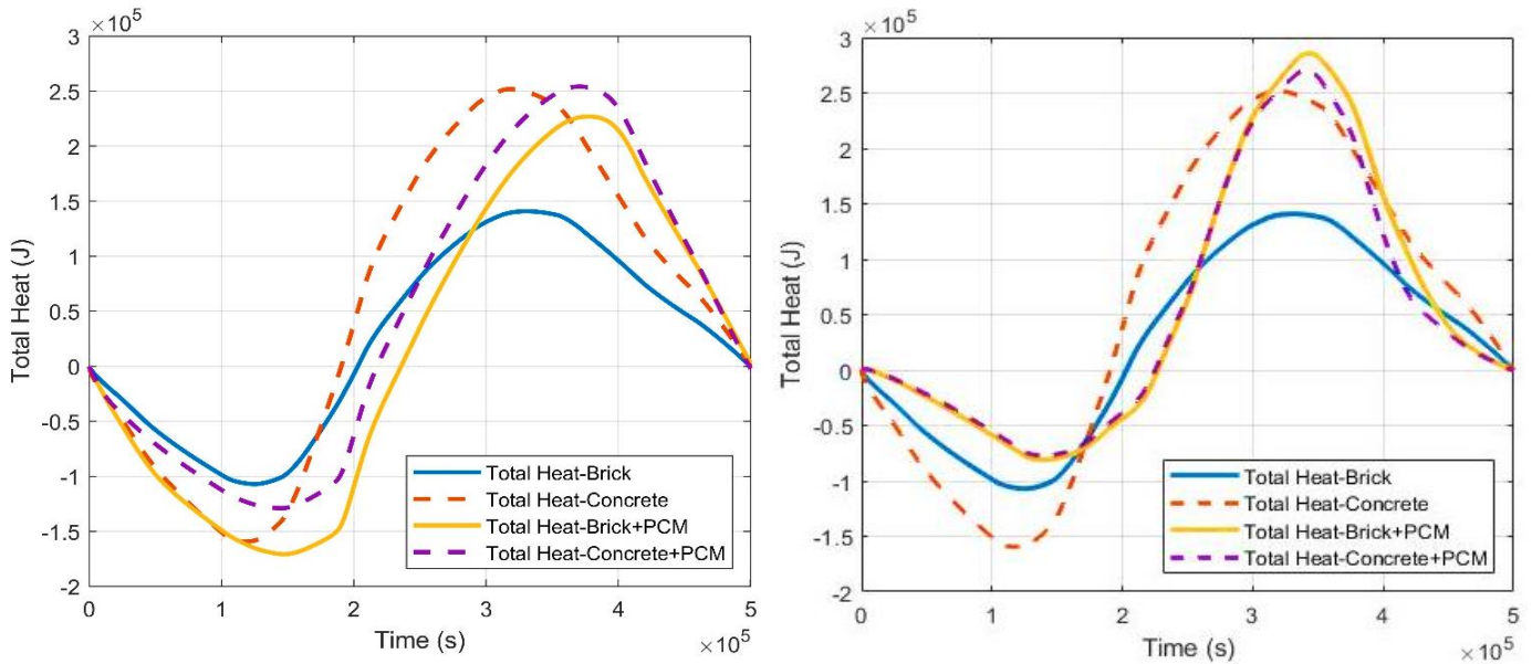
Figure 4.58. The total heat content in Case 2 with PCM1 (Left), PCM2 (Right)
