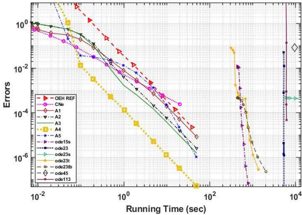
Figure 3.6. L_\infty errors as a function of the running time for the second (very stiff) system, in the case of the original OEH method (OEH REF), one stage CNe method, the new algorithms A1-A5 and different MATLAB routines.
