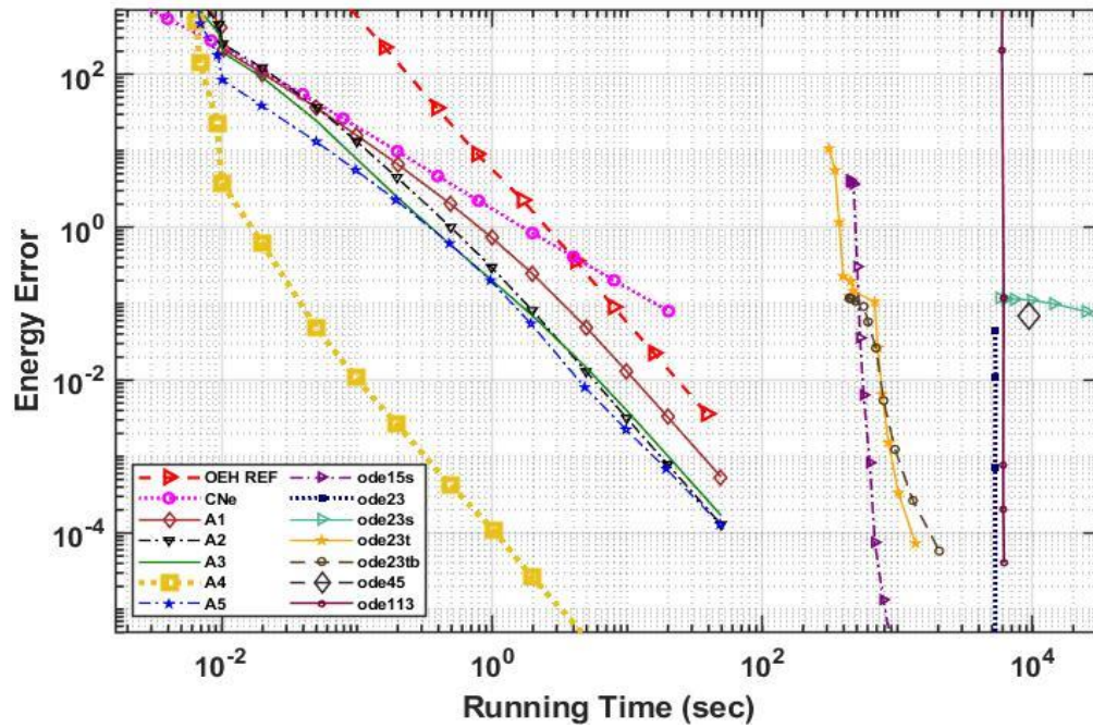
Figure 3.7. Energy errors as a function of the running time for the second (very stiff) system, in the case of the original OEH method (OEH REF), one stage CNe method, the new algorithms A1-A5 and different MATLAB routines.
