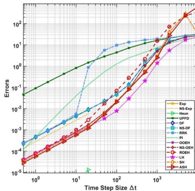
Figure 4.15. The maximum errors as a function of the time step size \Delta t for the equidistant mesh.
