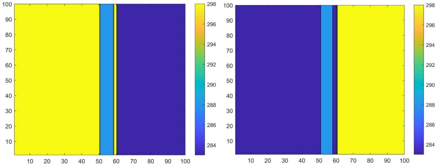
Figure 4.39. The contour of initial temperature distribution in Kelvin for free and forced convection in Case 3, in case of Cooling (left), and Heating (right).
