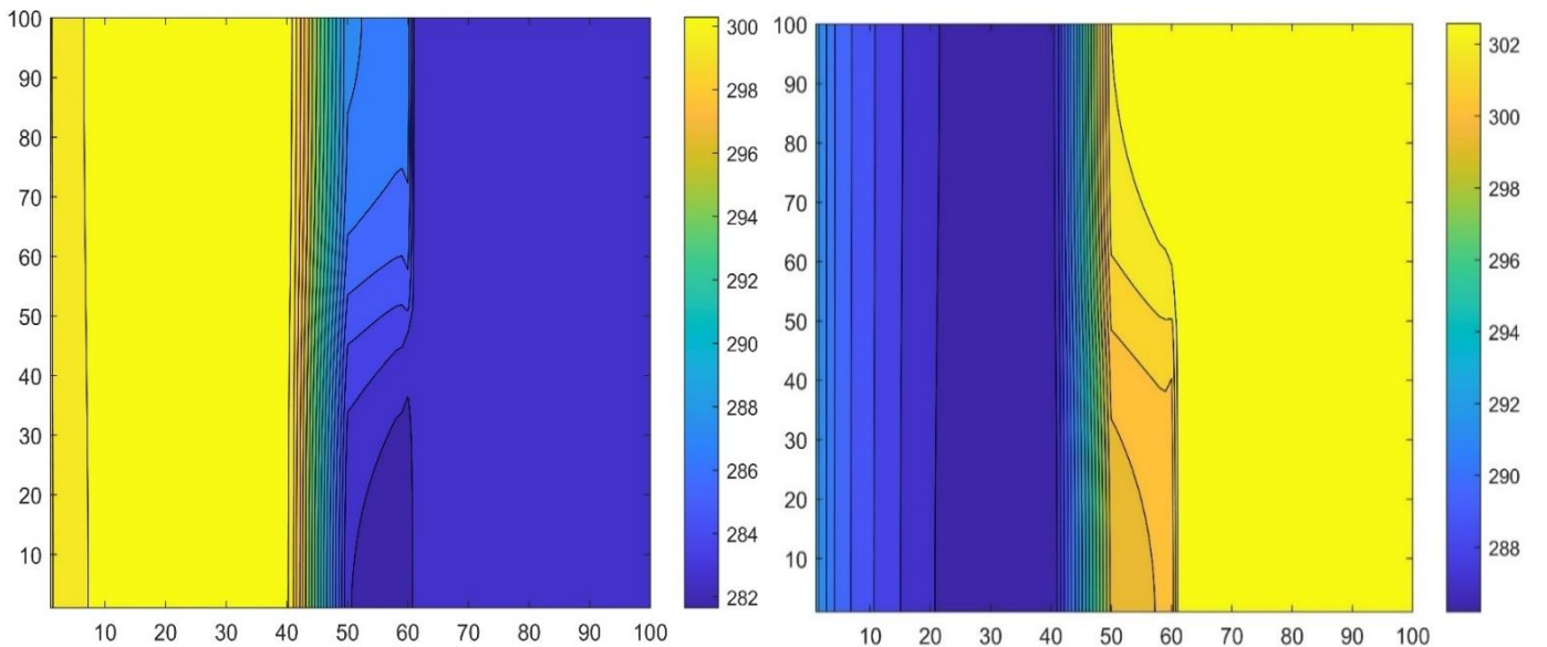
Figure 4.40. The contour of final temperature distribution in Kelvin for free-free convection in Case 3, in case of Cooling (left), and Heating (right).
