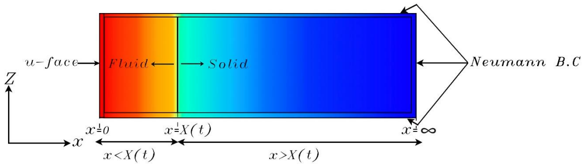
Figure 4.45. The paraffin wax inside the container
