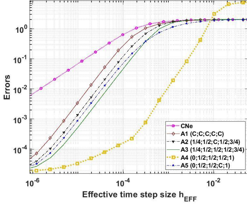
Figure 3.8. The L_\infty errors as a function of \Delta t_{\text{EFF}} for the u_2 solutions.
