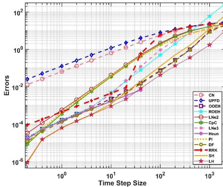
Figure 4.7. The maximum errors as a function of the time step size \Delta t for the equidistant mesh for a wall with insulation.
