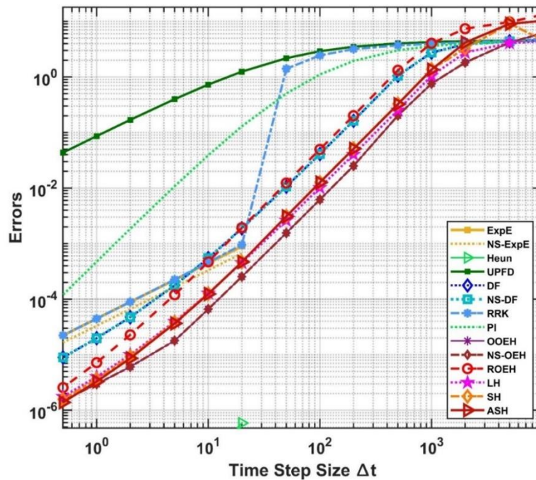
Figure 4.13. The maximum errors as a function of the time step size \Delta t for the 14 examined methods in the case of a surface area.
