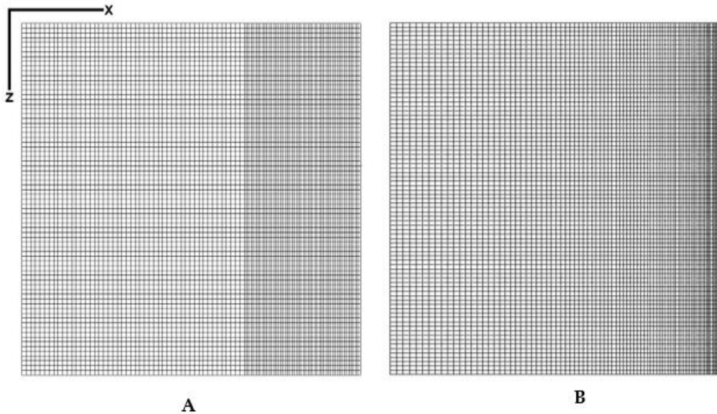
Figure 4.2. (A) Abrupt change. (B) Gradual change in the x direction.
