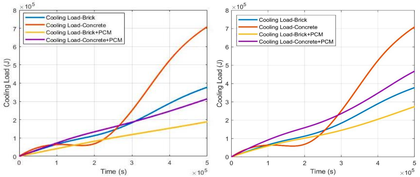
Figure 4.59. Cooling load in Case 1 with PCM1 (Left), PCM2 (Right)
