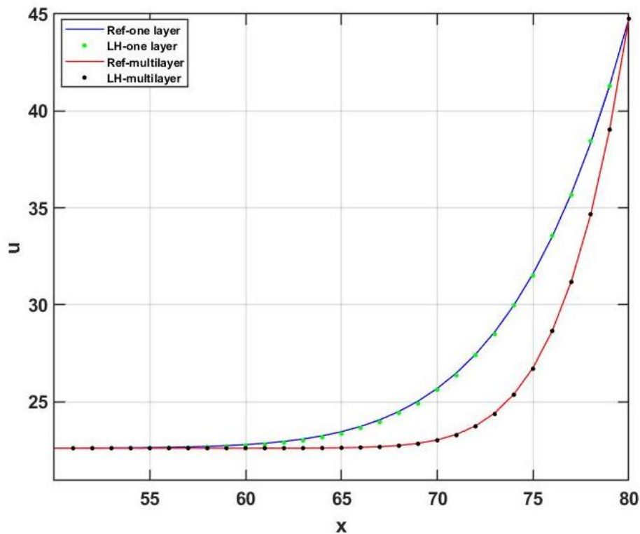
Figure 4.11. The temperature u °C as a function of the cell index in the x direction at the middle row ( z \approx 0.5 ) in the case of the reference solution (Ref) and the leapfrog-hopscotch (LH) method for \Delta t = 400 in the case of the one-layer wall and the insulated wall using an equidistant grid.
