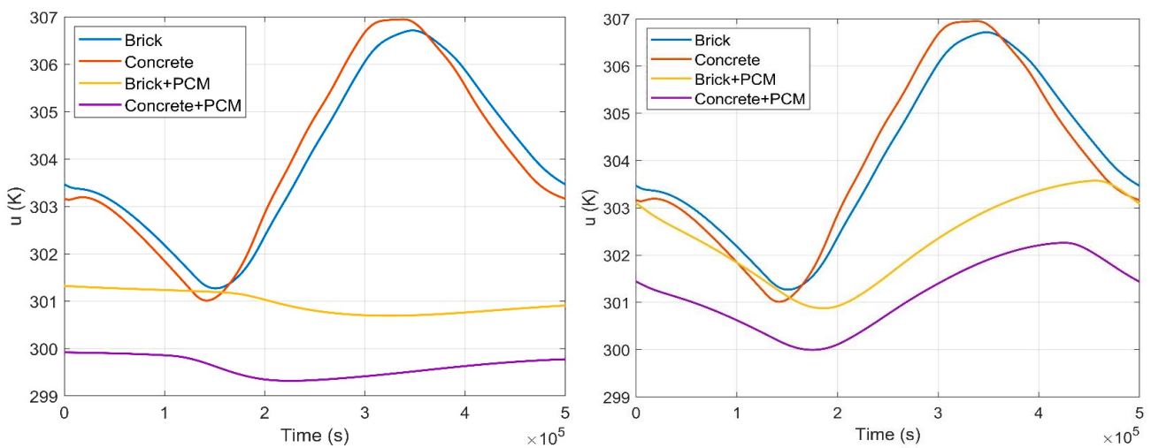
Figure 4.55. The temperature history in the middle of brick or concrete part in Case1 with PCM1 (Left), PCM2 (Right)
