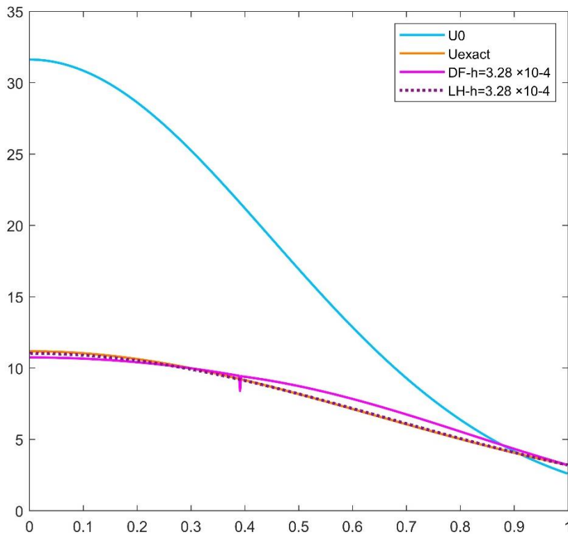
Figure 4.28. The values of temperature as a function of r variable in case of the initial function u^0 , the analytical solution U_{exact} , the DF method, and the LH method in case of spherical coordinates for a = 1.2 .
