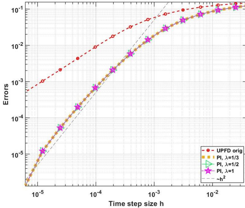
Figure 3.10. The L_\infty for the numerical solutions of the diffusion-reaction-radiation equation in the case of Algorithm 1 and the new pseudo-implicit Algorithm 3 for three different values of parameter \lambda .
