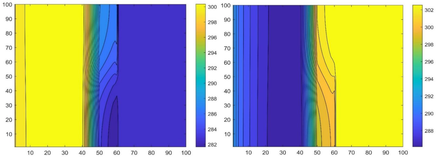
Figure 4.41. The contour of final temperature distribution in Kelvin for free-forced convection in Case 3, in case of Cooling (left), and Heating (right).
