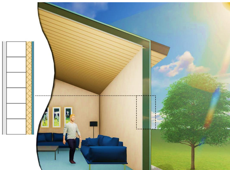
Figure 4.35. Visualization of the studied case, the selected wall cross-section
