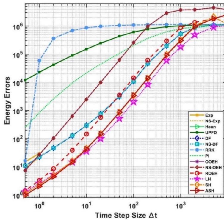
Figure 4.21. The energy errors as a function of the time step size for the non-equidistant mesh.
