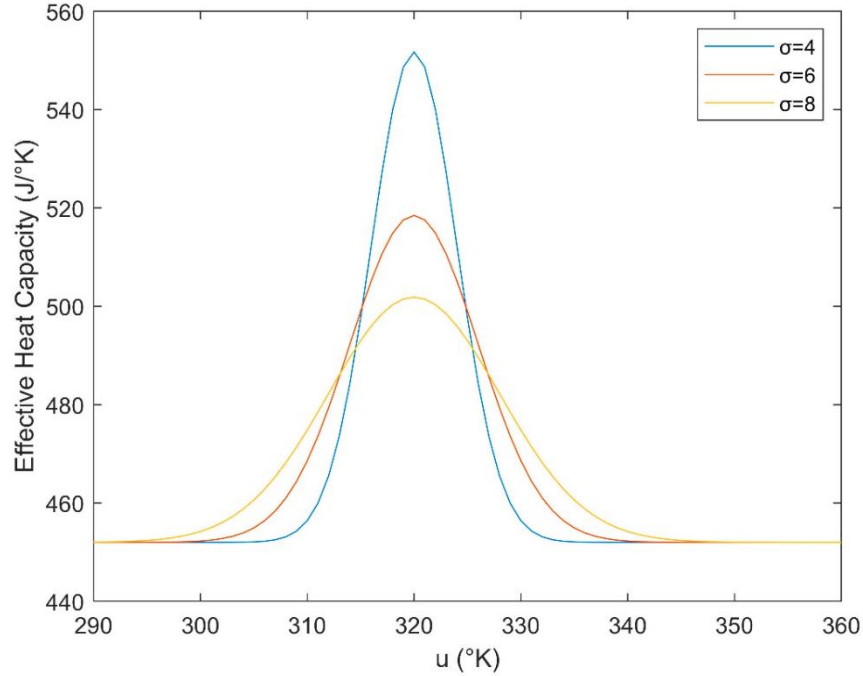
Figure 4.44. Gaussian function representative of the heat capacity with temperature
