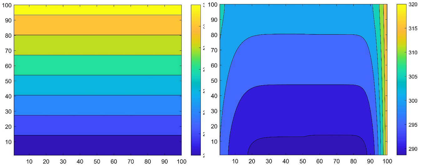
Figure 4.18. The temperature distribution contour in Kelvin for the equidistant mesh at initial (left) and final time (right), in the case of the multilayer cross-sectional area. The numbers on the vertical and horizontal axes of the contours are the indices of the cells.
