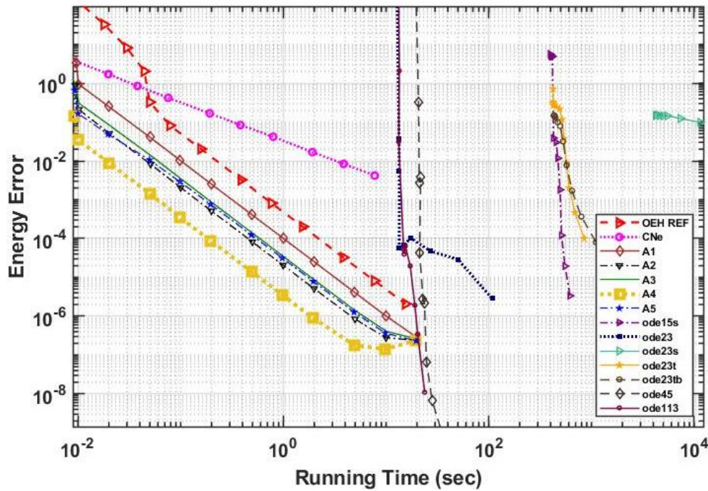
Figure 3.5. Energy errors as a function of the running time for the first (moderately stiff) system, in the case of the original OEH method (OEH REF), one stage CNe method, the new algorithms A1-A5 and different MATLAB routines.
