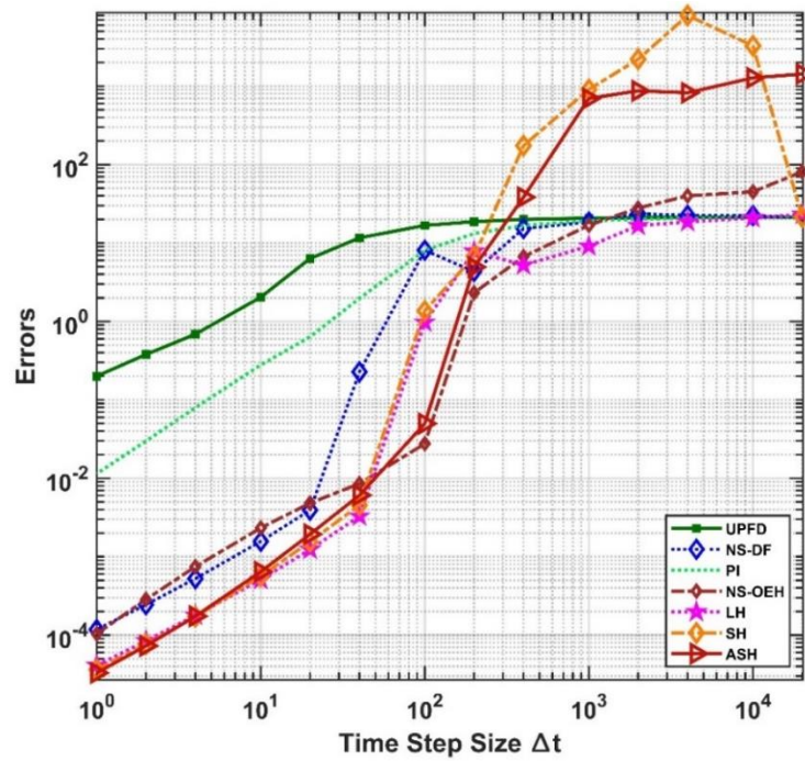
Figure 4.37. The maximum errors as a time step size function \Delta t for the 7 tested methods in the case of free-forced convection cooling in Case 3.
