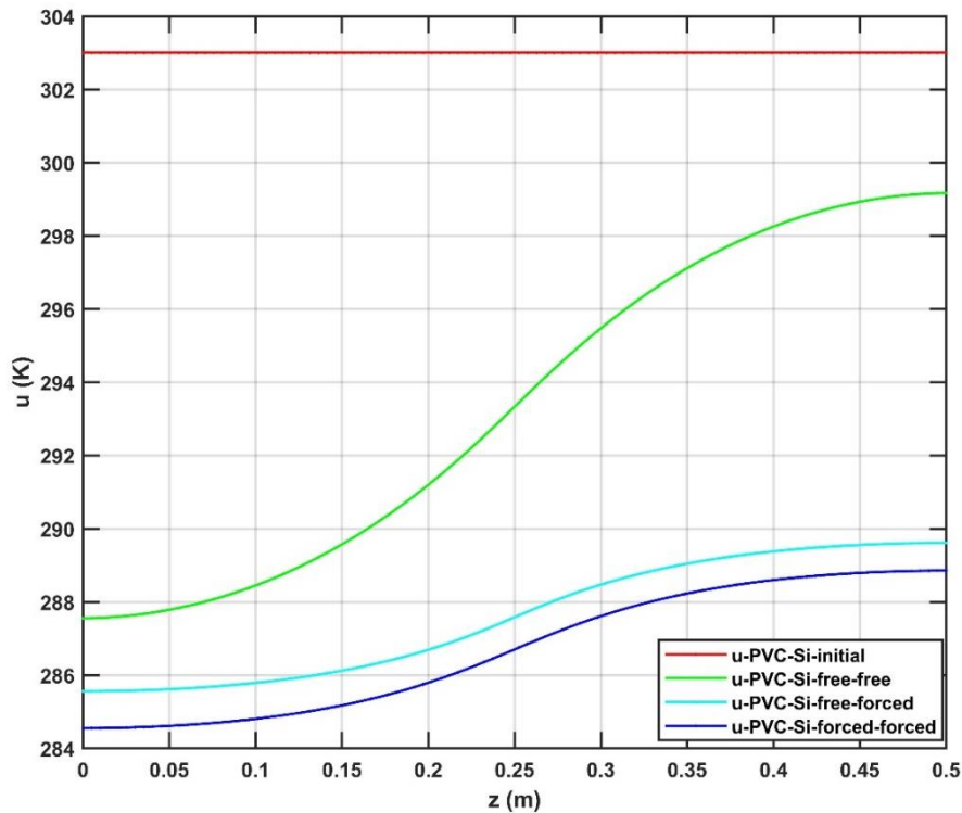
Figure 4.43. The temperature at the PVC (silicon) border in Kelvin for Case 3 in case of Cooling
