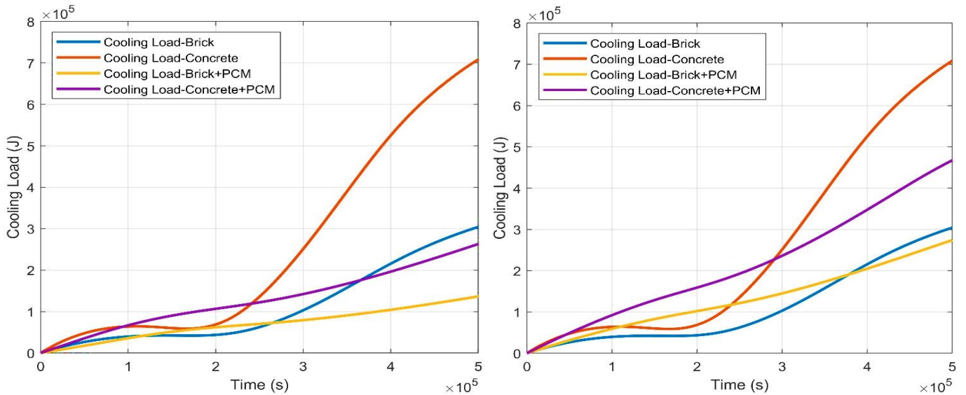
Figure 4.60. Cooling load in Case 2 with PCM1 (Left), PCM2 (Right)
