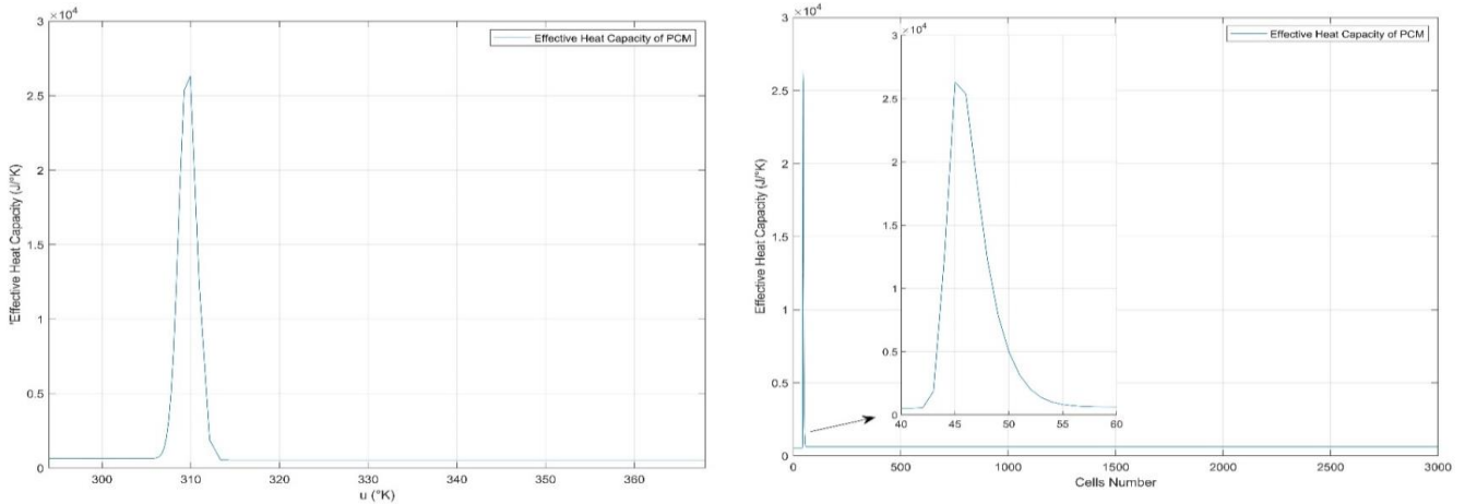
Figure 4.49. The EHC for Paraffin wax slab plotted with the final temperature u (left) and with Cell\ Number (right).
