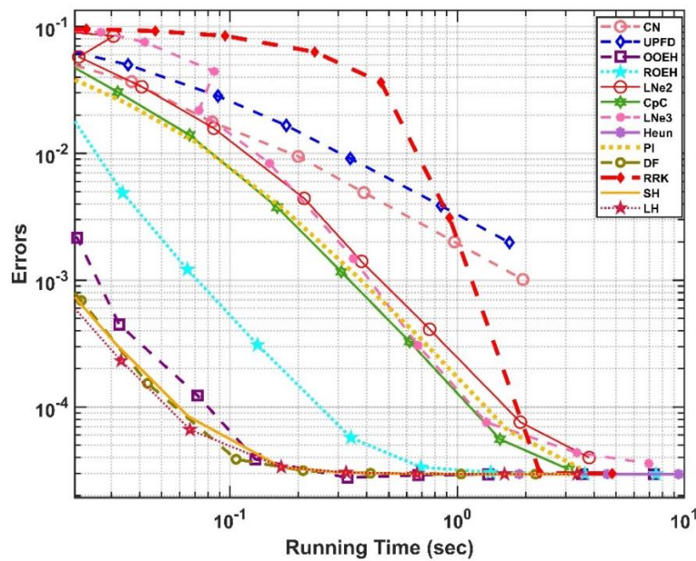
Figure 4.6. The maximum errors as a function of the running time for the abrupt change in the x -direction and gradual change in the z -direction.
