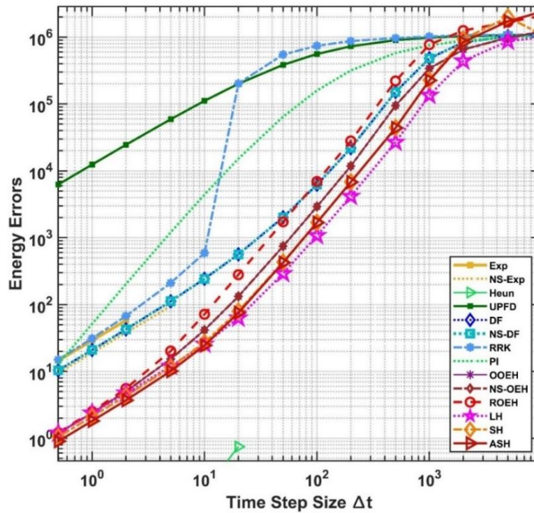
Figure 4.17. The energy errors as a function of the time step size \Delta t for the non-equidistant mesh
