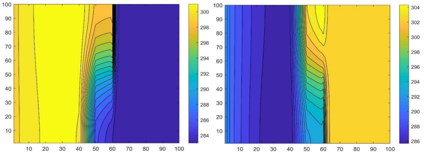
Figure 4.40. The contour of final temperature distribution in Kelvin for free-free convection in Case 3, in case of Cooling (left), and Heating (right).
