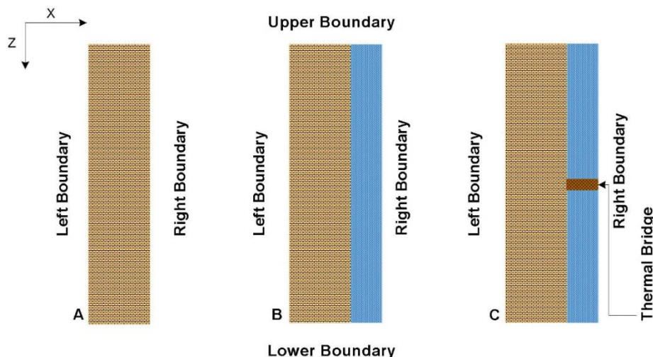
Figure 4.12. (A) One-layer wall, (B) wall with insulator, and (C) wall with insulator and thermal bridge.
