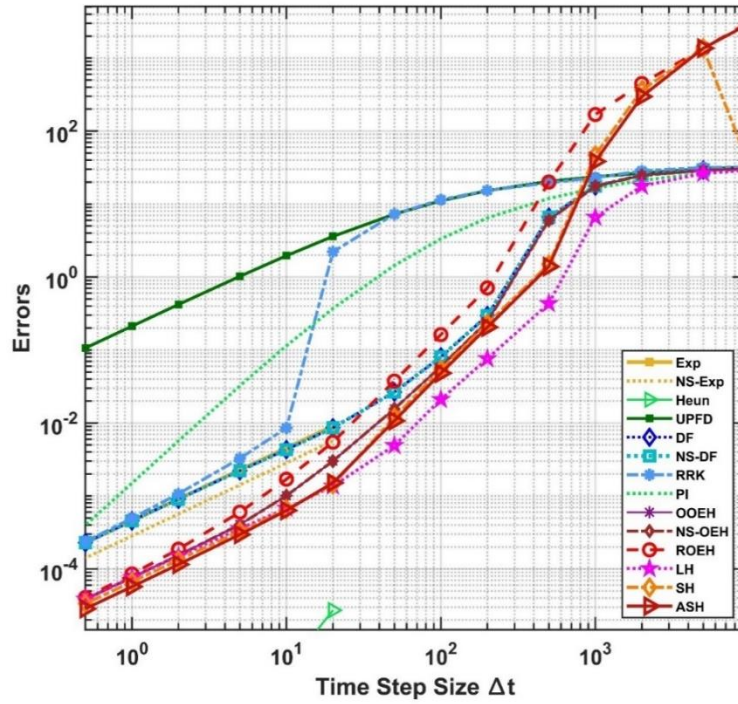
Figure 4.16. The maximum errors as a function of the time step size for the non-equidistant mesh.
