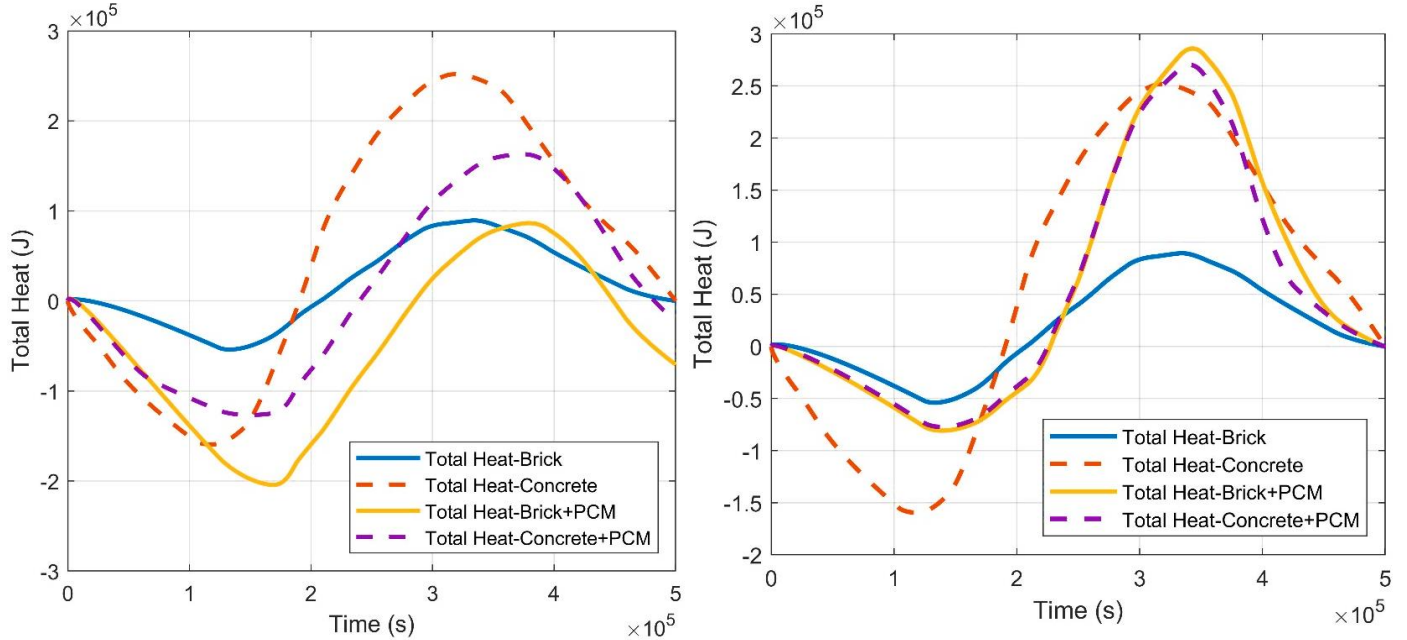
Figure 4.57. The total heat content in Case 1 with PCM1 (Left), PCM2 (Right)
