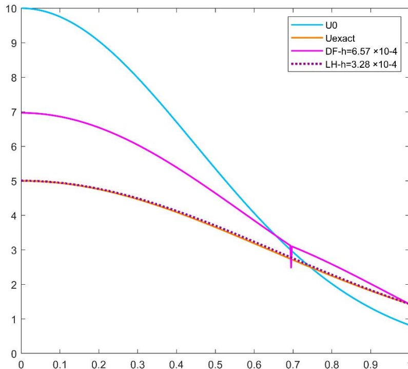
Figure 4.26. The values of temperature as a function of variable r in case of the initial function u^0 , the analytical solution U_{exact} , the DF method, and the LH method in case of cylindrical coordinates for a = 1 .
