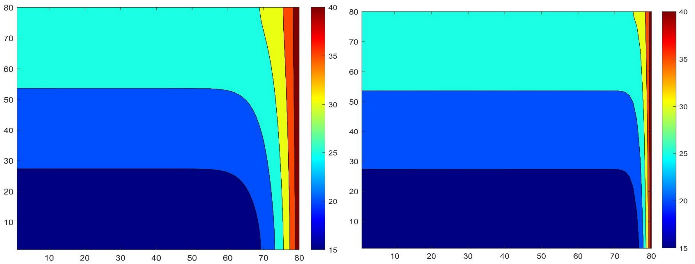
Figure 4.10. The temperature distribution contour for the equidistant mesh at the final time in case of: a wall (left), and a wall with insulation (Right)
