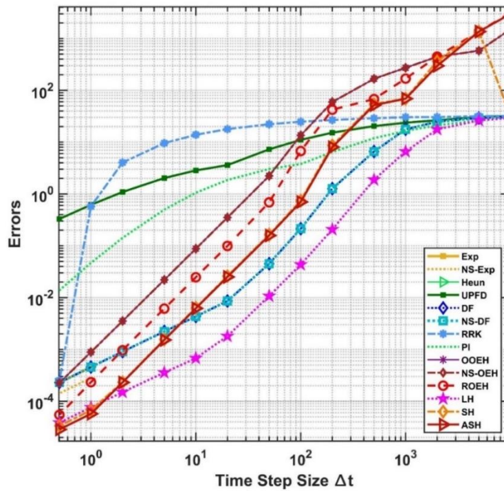
Figure 4.20. The maximum errors as a function of the time step size for the non-equidistant mesh.
