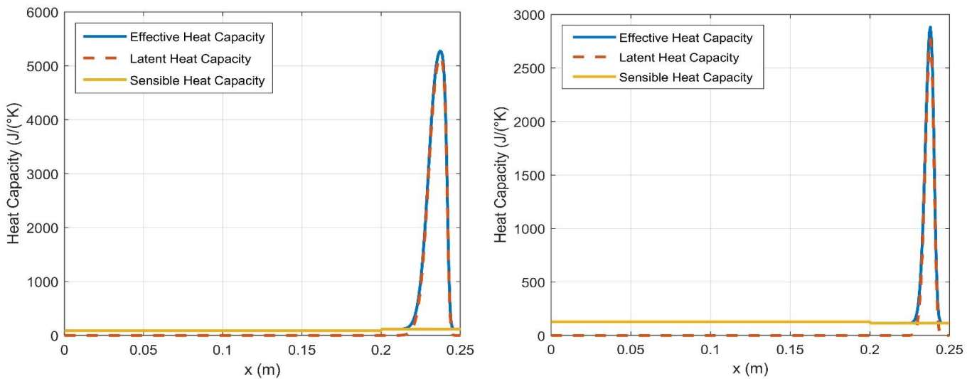
Figure 4.52. The heat capacity in Case1 for of Brick+PCM1 (Left), Concrete +PCM1 (Right)
