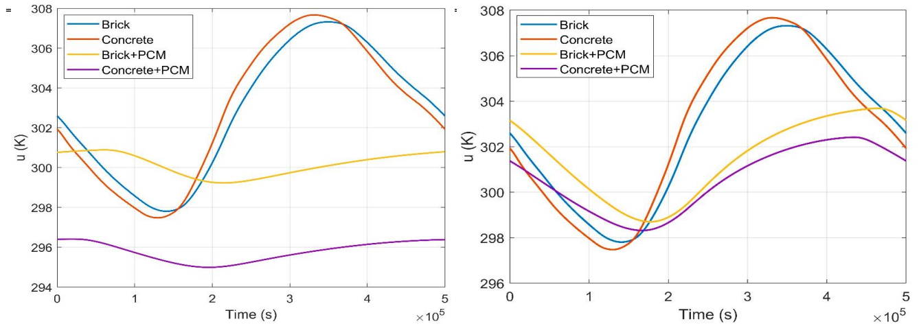
Figure 4.56. The temperature history in the middle of brick or concrete part in Case2 with PCM1 (Left), PCM2 (Right)
