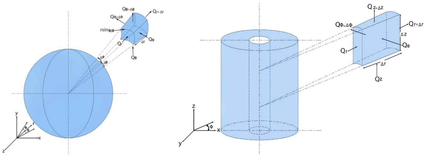
Figure 2.3. The cylindrical (left) and spherical (right) elements
