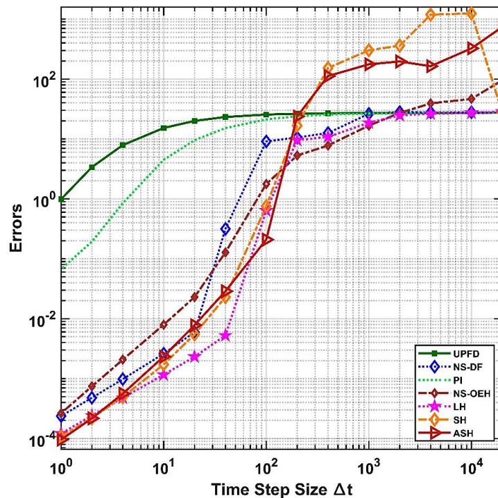
Figure 4.36. The maximum errors as a time step size function \Delta t for the 7 tested methods in the case free-free convection cooling in Case 3.
