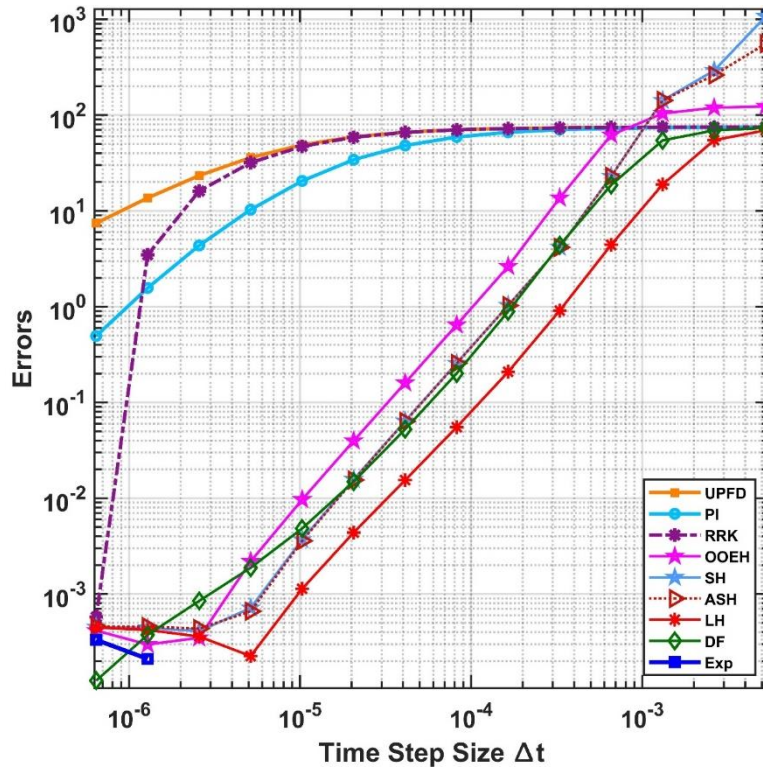
Figure 4.25. The maximum errors as a function of the time step size for the 9 numerical methods in case of cylindrical coordinates for a = 2 .
