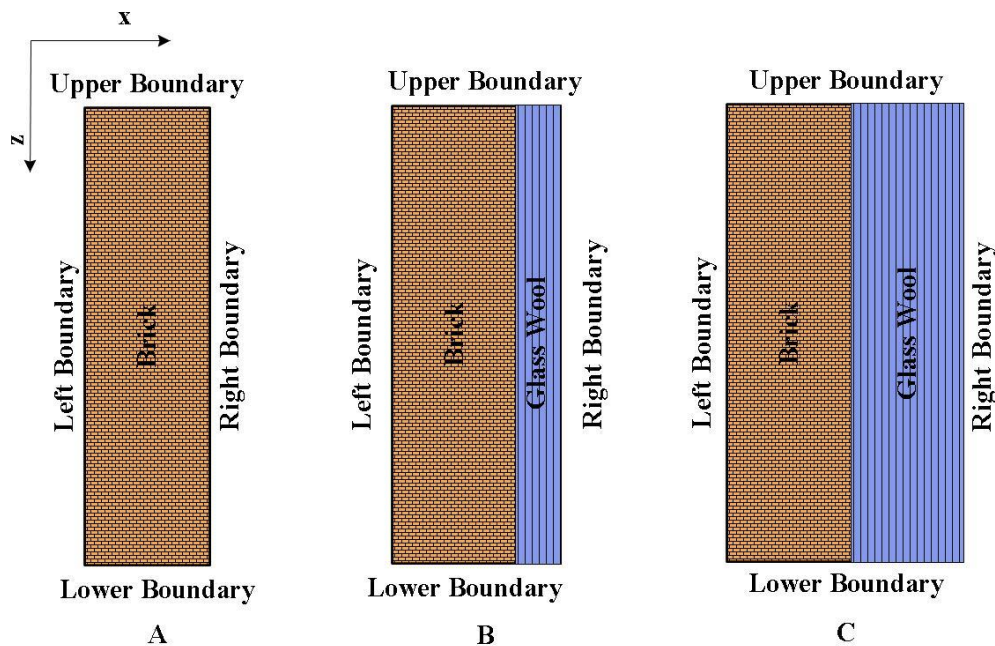
Figure 4.1. (A) One-layer wall, (B) and (C) wall with insulator.
