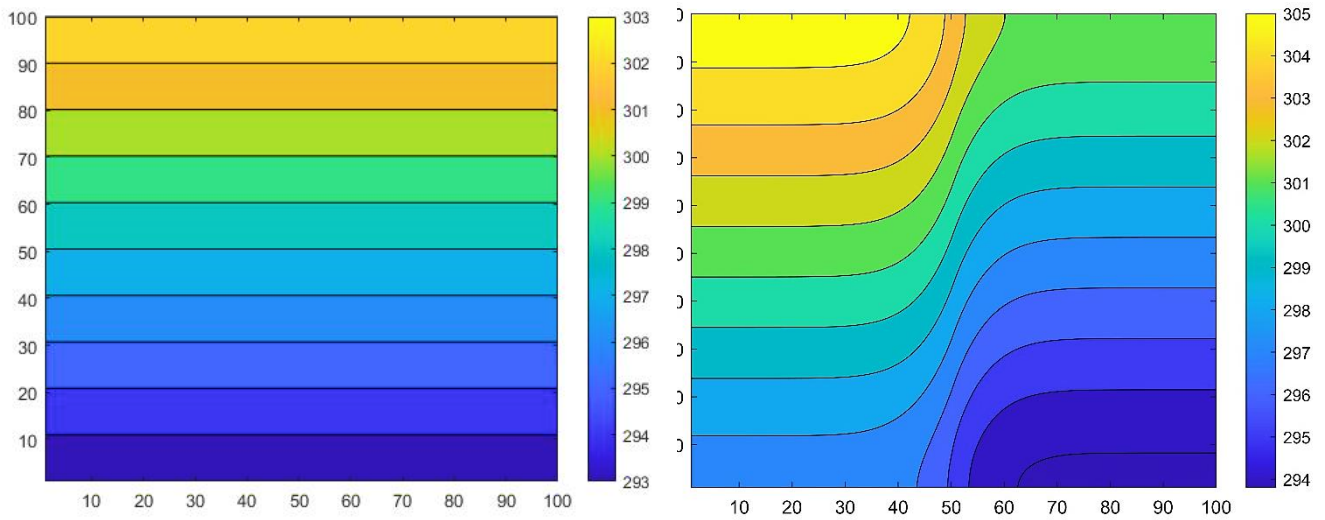
Figure 4.14. The temperature distribution contour in Kelvin for the equidistant mesh at initial (left) and final time (right), in the case of multilayer cross-sectional area. The numbers on the vertical and horizontal axes of the contours are the indices of the cells, which are the same as the coordinates in cm units.
