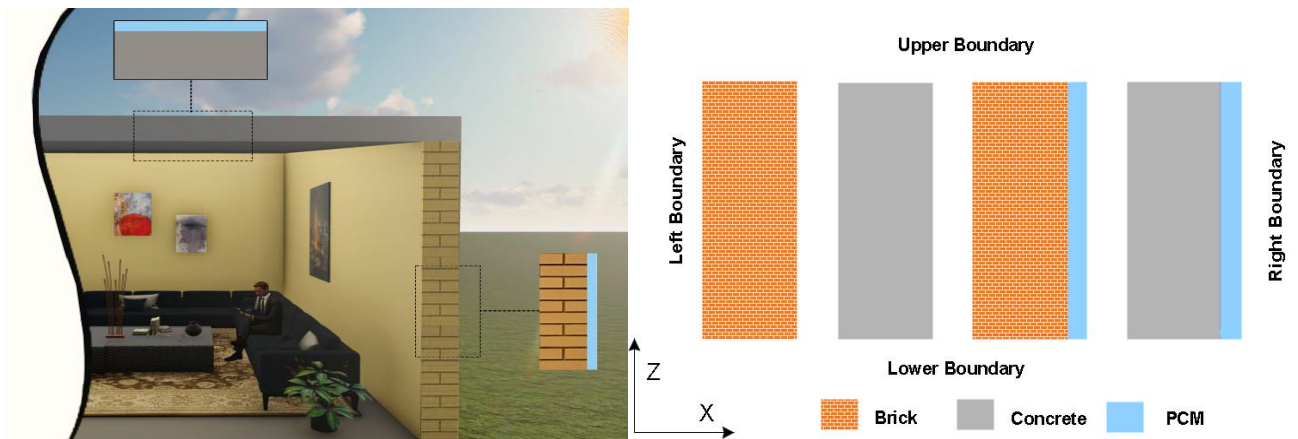
Figure 4.46. The selected section geometries of studies
