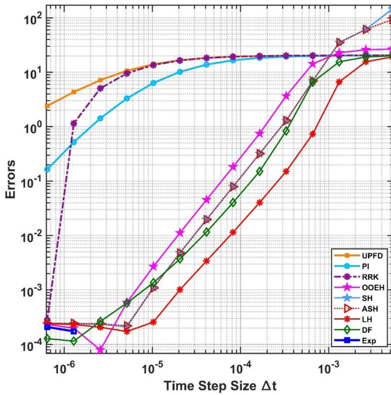
Figure 4.27. The maximum errors as a function of the time step size for the 9 numerical methods in the case of spherical coordinates for a = 1.2 .
