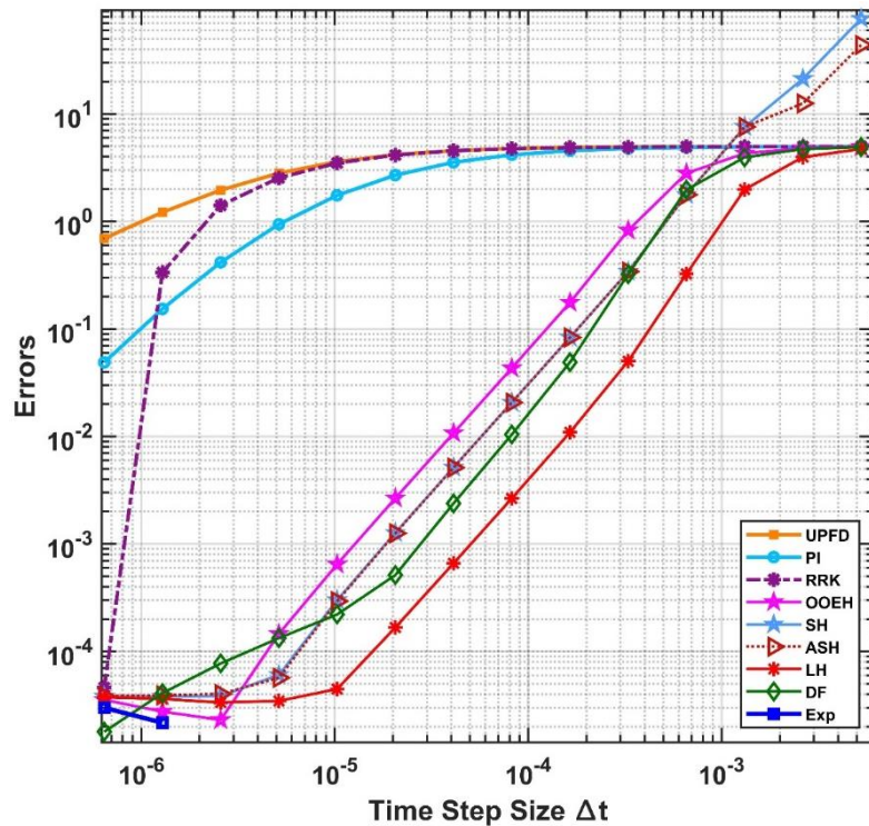
Figure 4.24. The maximum errors as a function of the time step size for the 9 numerical methods in case of cylindrical coordinates for a = 1 .
