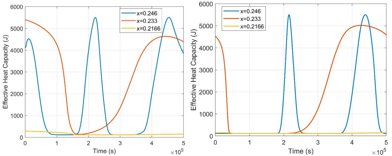
Figure 4.54. The Effective Heat Capacity history through PCM for Brick+ PCM1 in Case1 (Left), and Case2 (Right).
