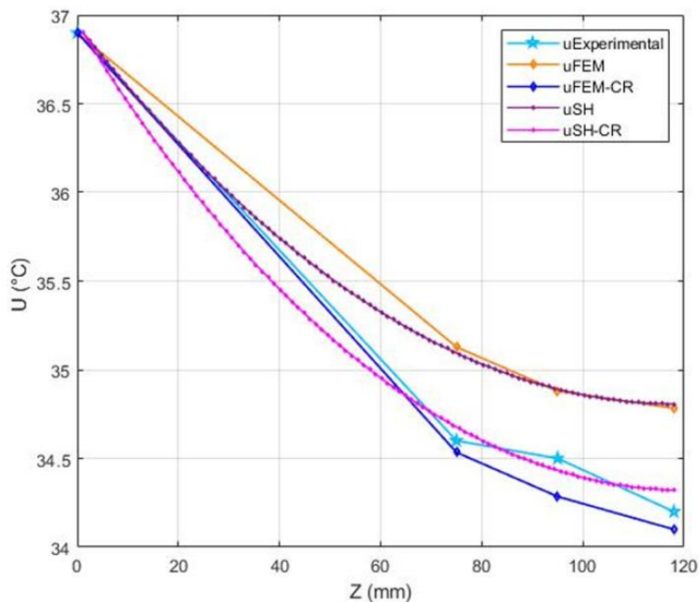
Figure 4.32. The temperature at the 4 selected measurement points in z at time t = 20 min.
