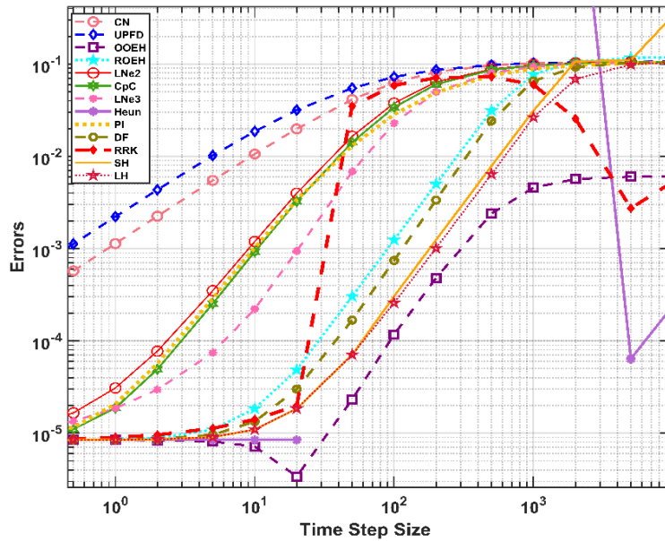
Figure 4.3. The maximum errors as a function of the time step size \Delta t for the 13 examined methods in the case of an equidistant mesh.
