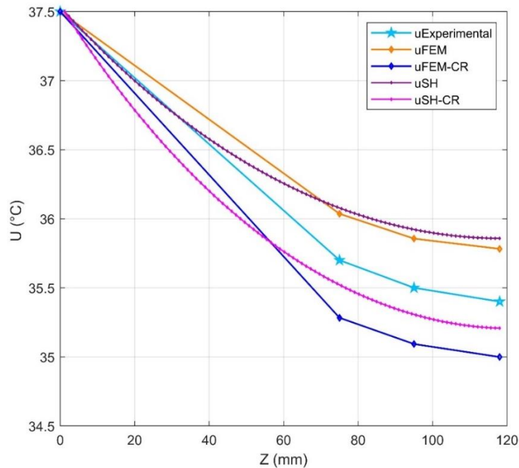
Figure 4.34. The temperature at the 4 selected measurement points in z at time t = 30 min.
