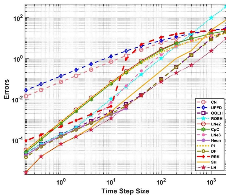
Figure 4.8. The maximum errors as a function of the time step size \Delta t for the non-equidistant mesh for a wall with insulation.
