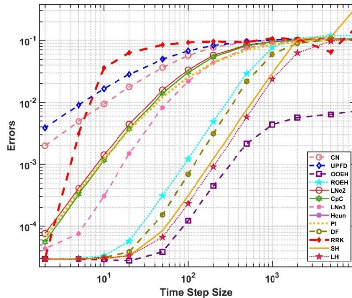
Figure 4.4. The maximum errors as a function of the time step size \Delta t for the abrupt change in the x -direction and gradual change in the z -direction.
